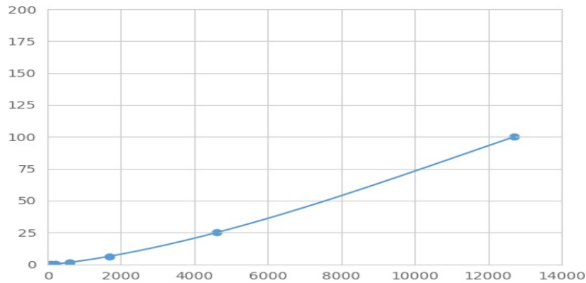
Typical Standard Curve for IDUa Magnetic Luminex Assay.
