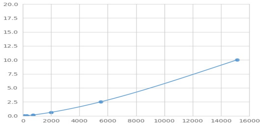
Typical Standard Curve for IMMP2L Magnetic Luminex Assay.
