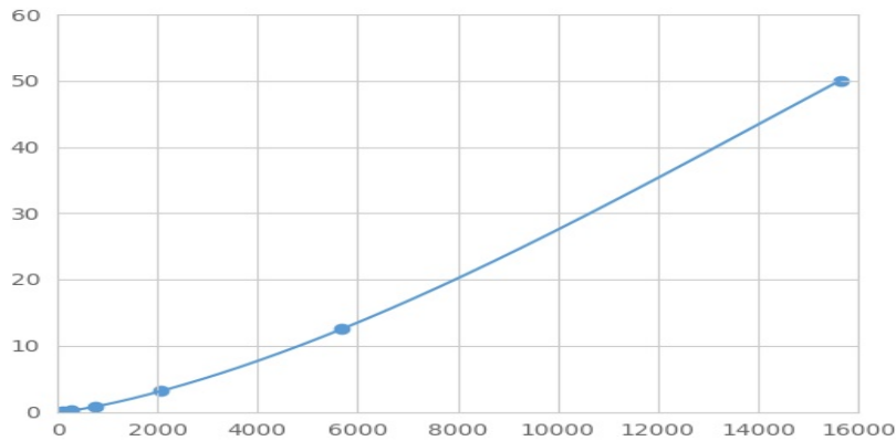
Typical Standard Curve for IMPDH2 Magnetic Luminex Assay.
