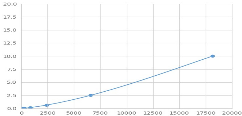
Typical Standard Curve for ITGa9 Magnetic Luminex Assay.
