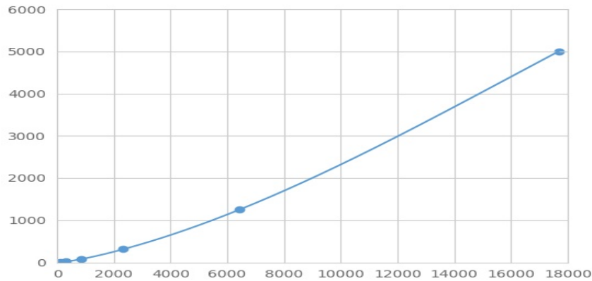
Typical Standard Curve for IFI35 Magnetic Luminex Assay.
