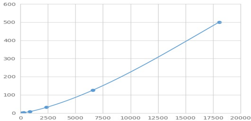
Typical Standard Curve for IL1F9 Magnetic Luminex Assay.
