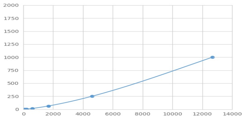
Typical Standard Curve for JAM3 Magnetic Luminex Assay.
