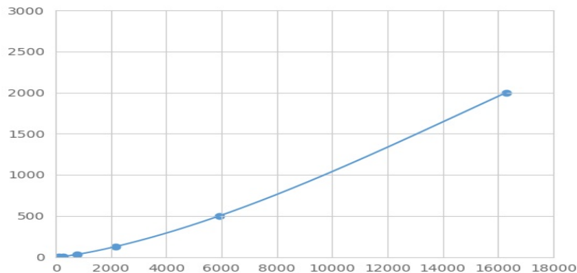
Typical Standard Curve for KLK6 Magnetic Luminex Assay.
