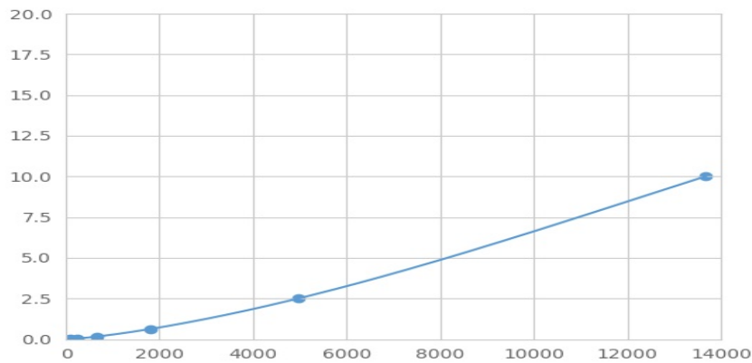
Typical Standard Curve for KLK9 Magnetic Luminex Assay.
