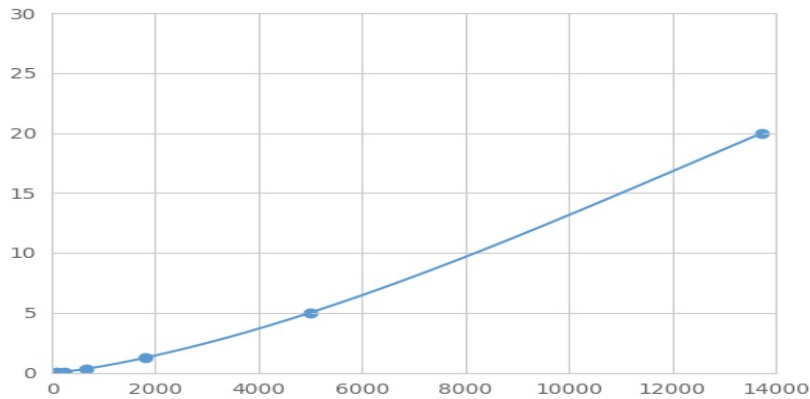
Typical Standard Curve for y+LAT1 Magnetic Luminex Assay.
