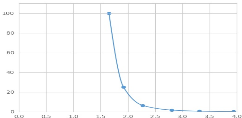
Typical Standard Curve for LNG Magnetic Luminex Assay.
