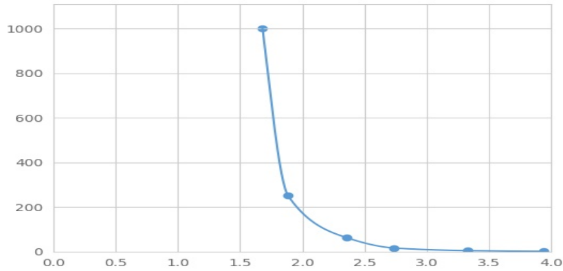
Typical Standard Curve for LRT Magnetic Luminex Assay.
