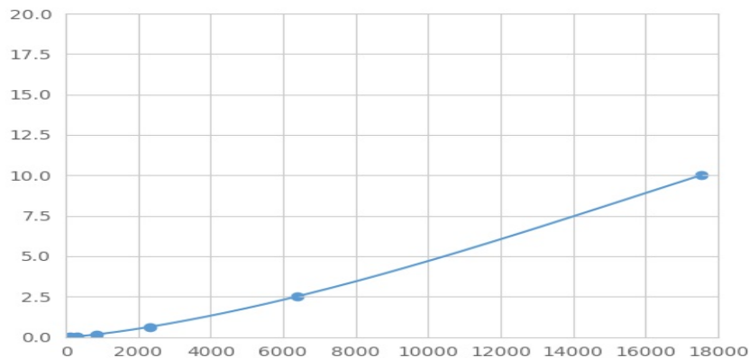
Typical Standard Curve for LRH1 Magnetic Luminex Assay.
