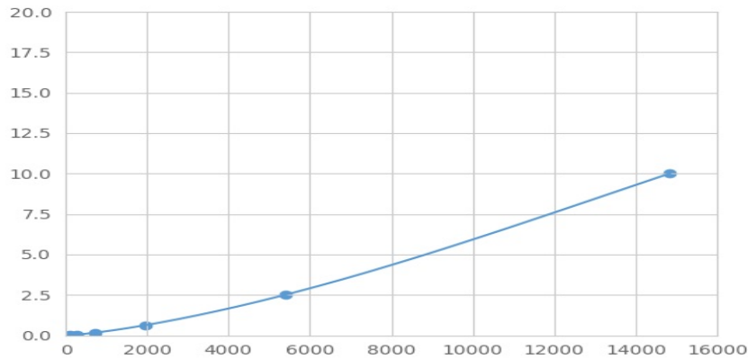
Typical Standard Curve for LASS6 Magnetic Luminex Assay.
