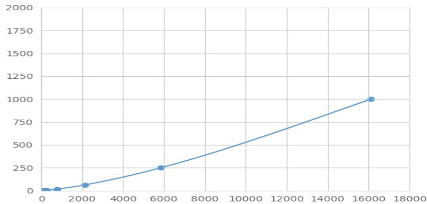
Typical Standard Curve for MIP1g Magnetic Luminex Assay.
