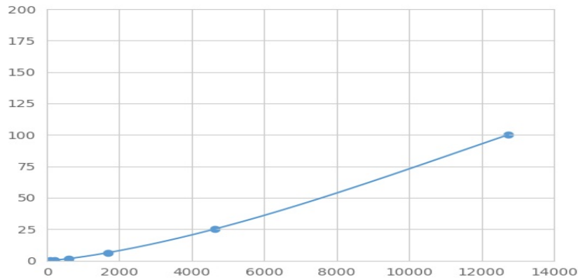
Typical Standard Curve for MGAM Magnetic Luminex Assay.
