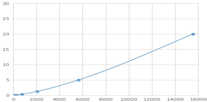
Typical Standard Curve for MMP13 Magnetic Luminex Assay.
