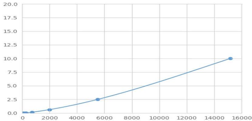
Typical Standard Curve for MMP26 Magnetic Luminex Assay.
