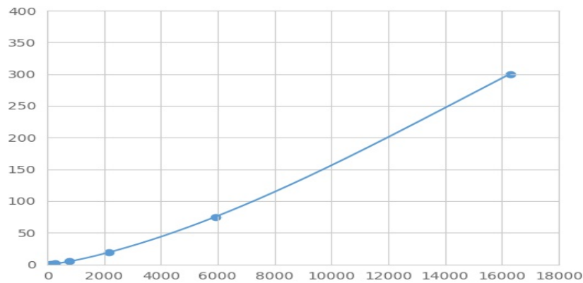
Typical Standard Curve for MMP9 Magnetic Luminex Assay.
