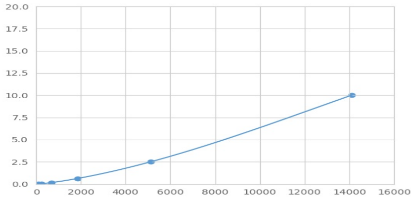
Typical Standard Curve for MTNR1A Magnetic Luminex Assay.
