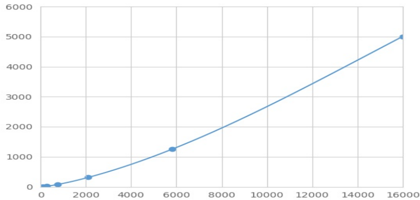
Typical Standard Curve for MTA1 Magnetic Luminex Assay.
