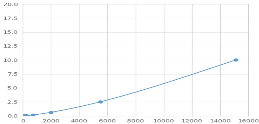
Typical Standard Curve for MAP2 Magnetic Luminex Assay.
