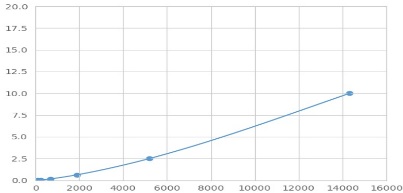
Typical Standard Curve for MR Magnetic Luminex Assay.
