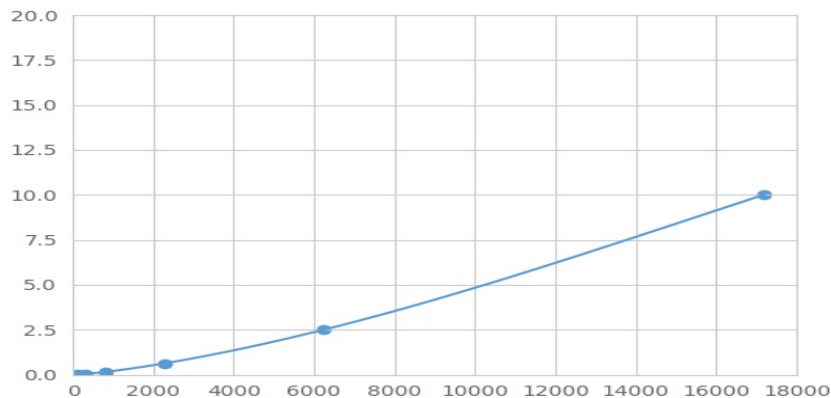
Typical Standard Curve for MOGAT2 Magnetic Luminex Assay.
