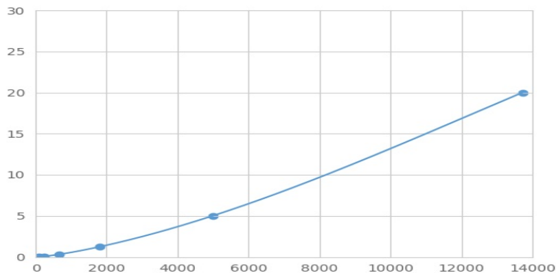
Typical Standard Curve for MMRN2 Magnetic Luminex Assay.
