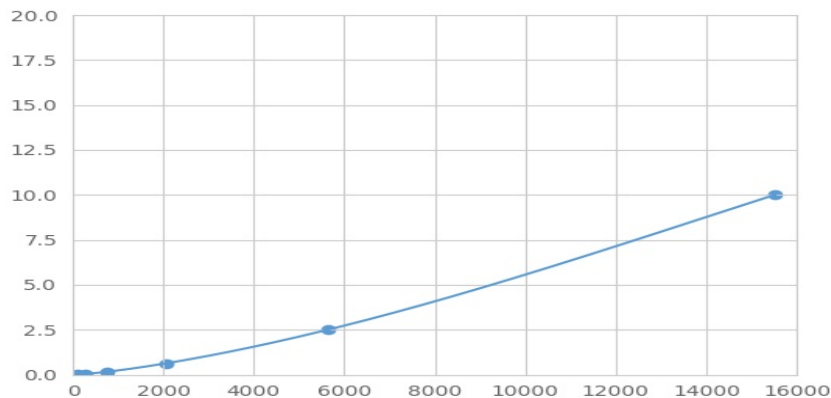
Typical Standard Curve for MUTYH Magnetic Luminex Assay.
