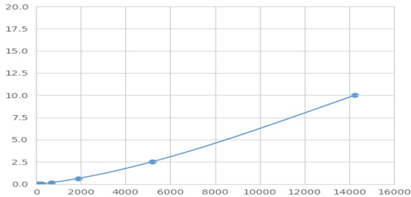
Typical Standard Curve for MyoD Magnetic Luminex Assay.
