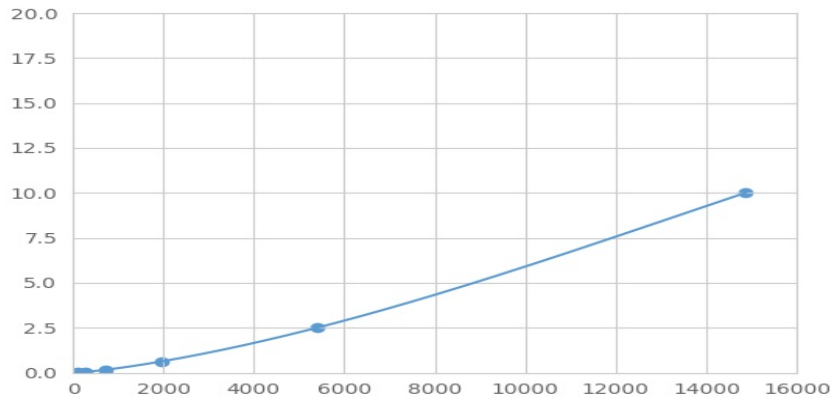
Typical Standard Curve for MYH1 Magnetic Luminex Assay.
