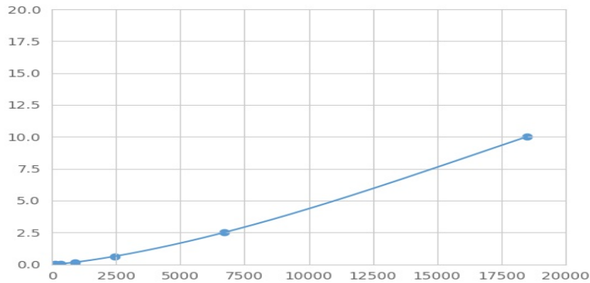
Typical Standard Curve for NPR3 Magnetic Luminex Assay.
