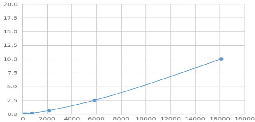
Typical Standard Curve for NGF Magnetic Luminex Assay.
