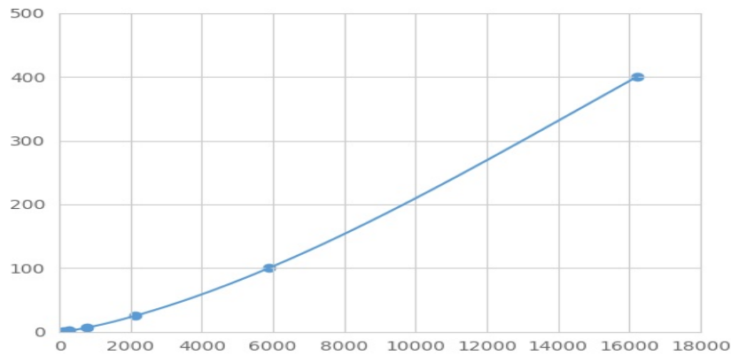
Typical Standard Curve for SELP Magnetic Luminex Assay.
