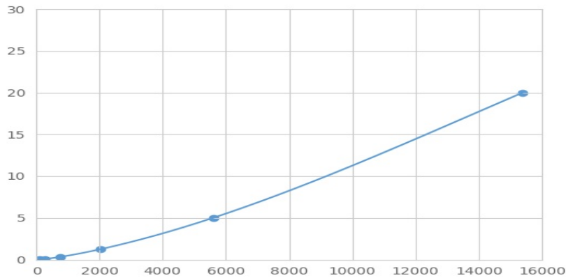
Typical Standard Curve for PEBP4 Magnetic Luminex Assay.
