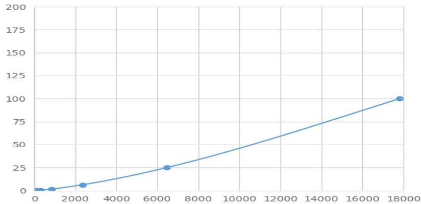
Typical Standard Curve for PFKL Magnetic Luminex Assay.
