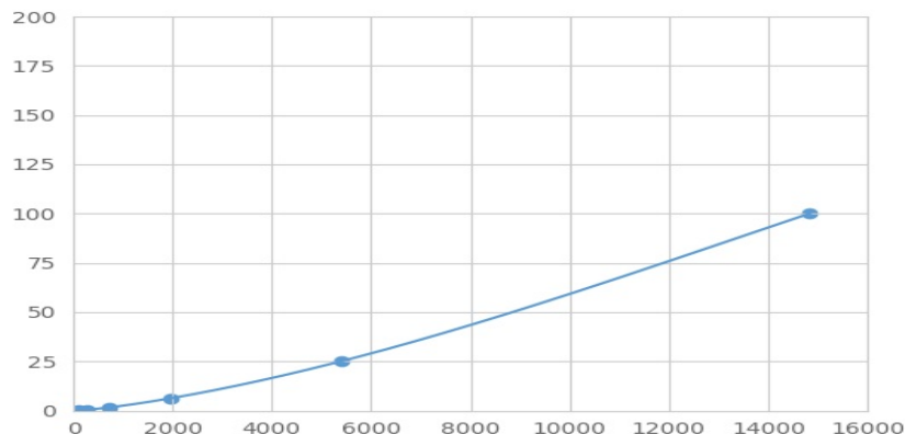
Typical Standard Curve for PLD2 Magnetic Luminex Assay.
