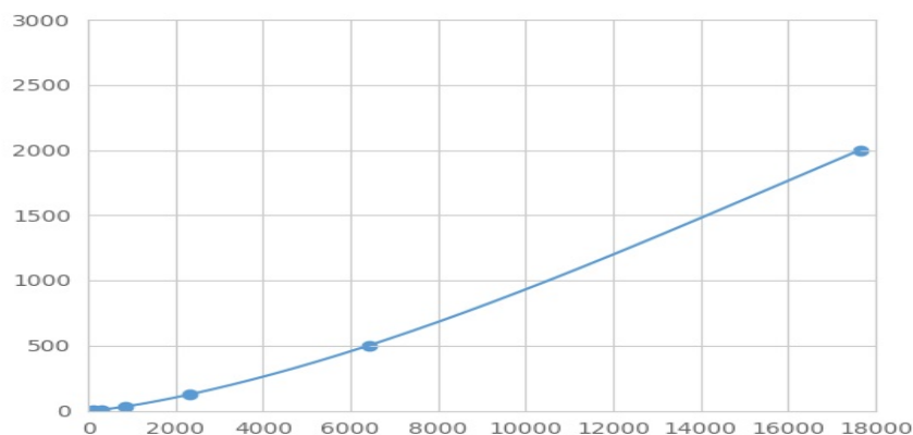
Typical Standard Curve for PDGFC Magnetic Luminex Assay.
