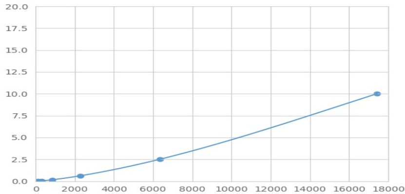
Typical Standard Curve for PLAGL2 Magnetic Luminex Assay.
