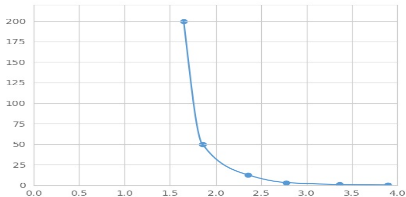
Typical Standard Curve for PGI2 Magnetic Luminex Assay.
