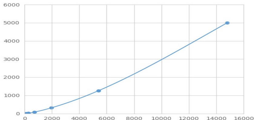
Typical Standard Curve for PTGDS Magnetic Luminex Assay.
