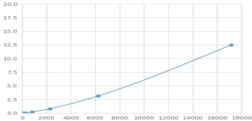
Typical Standard Curve for PSA Magnetic Luminex Assay.
