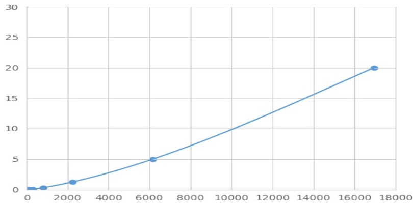
Typical Standard Curve for PAR4 Magnetic Luminex Assay.
