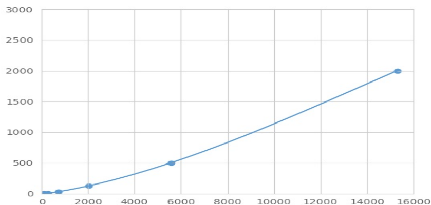
Typical Standard Curve for PCI Magnetic Luminex Assay.
