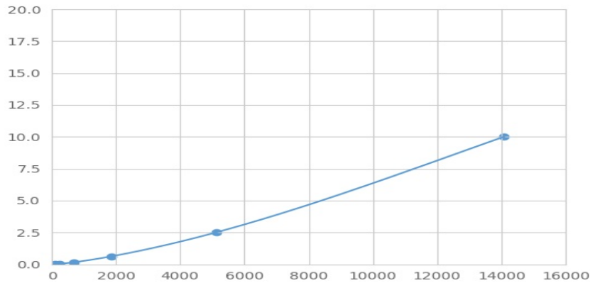
Typical Standard Curve for PICK1 Magnetic Luminex Assay.
