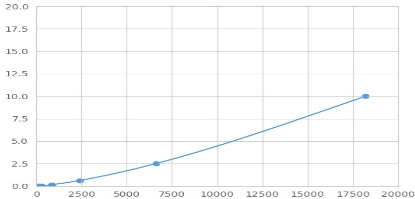
Typical Standard Curve for PRKACa Magnetic Luminex Assay.
