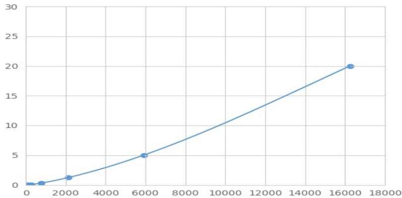
Typical Standard Curve for PRKG2 Magnetic Luminex Assay.
