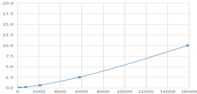
Typical Standard Curve for PKR Magnetic Luminex Assay.
