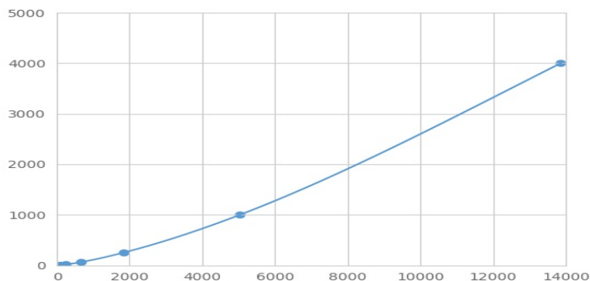
Typical Standard Curve for PROS Magnetic Luminex Assay.
