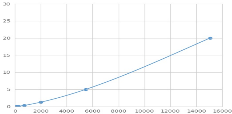
Typical Standard Curve for RAD51 Magnetic Luminex Assay.
