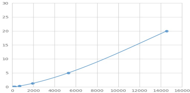
Typical Standard Curve for RCN3 Magnetic Luminex Assay.
