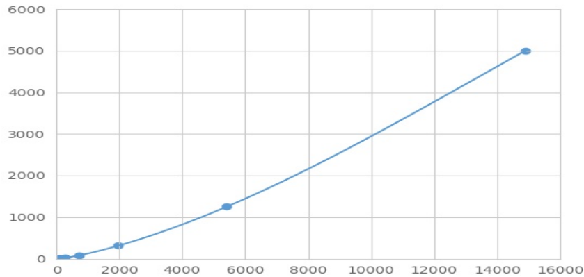
Typical Standard Curve for RXRa Magnetic Luminex Assay.
