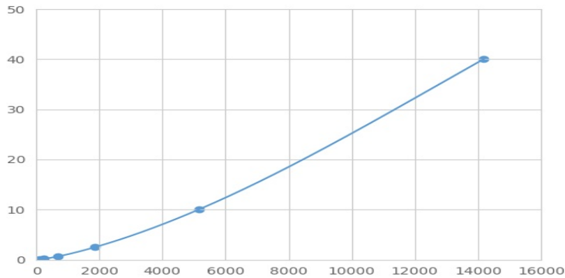
Typical Standard Curve for ARHGD1b Magnetic Luminex Assay.
